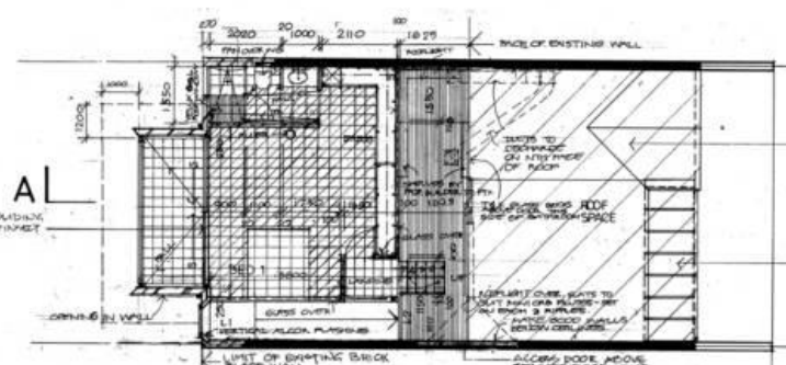
PLAN LEVEL 3
